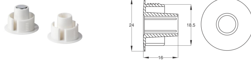
MK-3000-15
